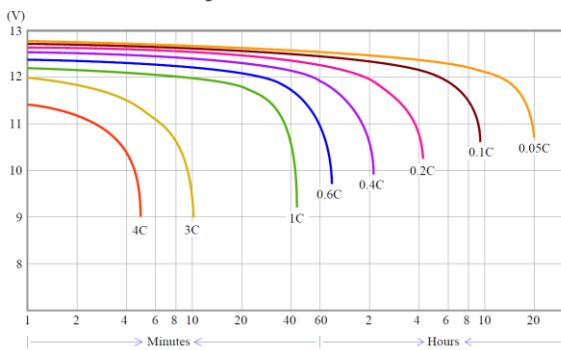
放電曲線 Discharge Characteristics Curves at 25°C
